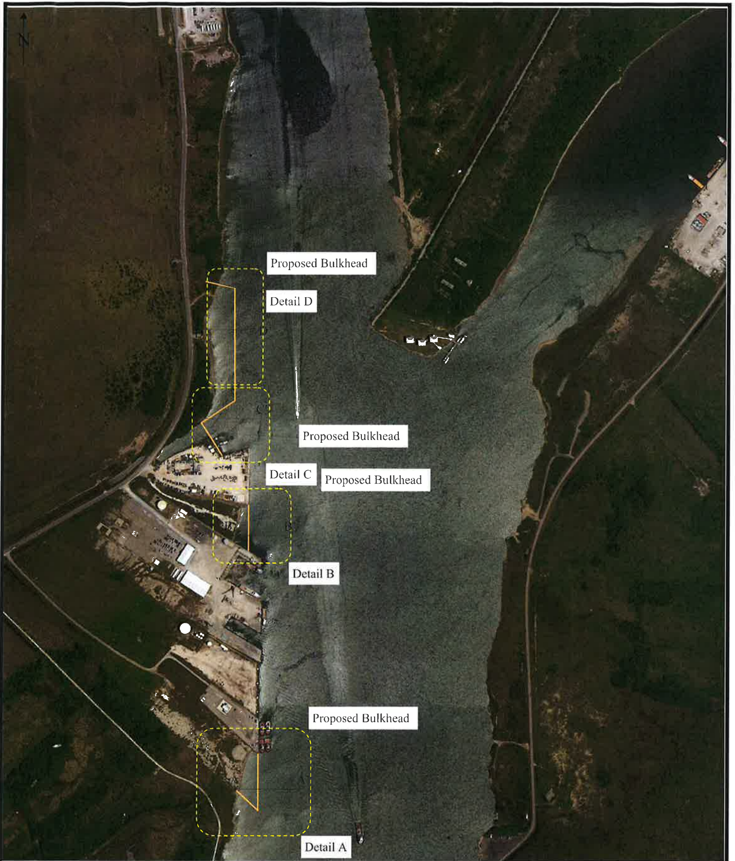
Figure 2. Plan View of Proposed Bulkhead Completion Project Revised M & C Oilfield Services, LLC. 5/30/2016
