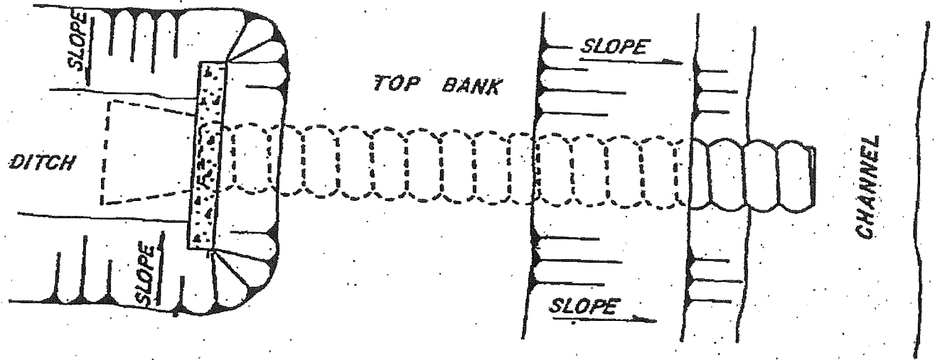
PLAN VIEW NO SCALE
