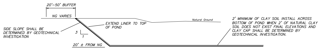
TYPICAL SECTION OF POND
